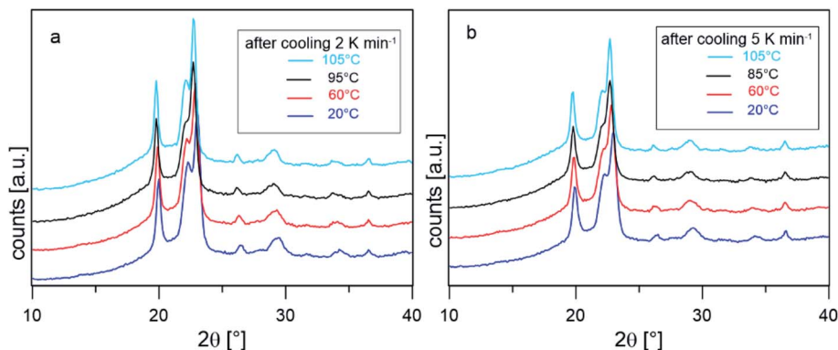
Fig. 4 XRD scans collected in situ at the indicated temperature after cooling from the melt at 2 \text{ K min}^{-1} (a) and 5 \text{ K min}^{-1} (b).
