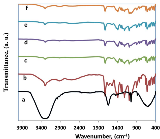
Fig. 2 FT-IR spectra for (a) garlic extract, (b) CMC/AG/GL blend, (c) CMC/AG/GL/TiO 2 bionanocomposites as well as the CMC/AG/GL/GE-TiO 2 bionanocomposites containing different ratios of garlic extract, (d) 2%, (e) 4%, and (f) 8%.
