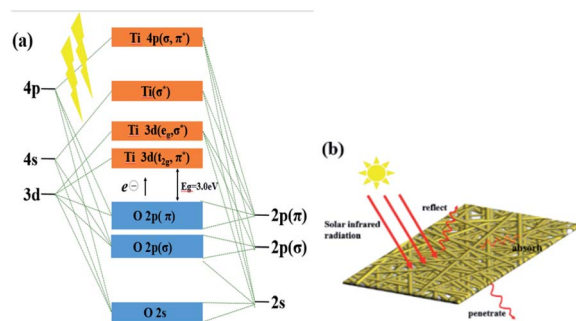
Fig. 7 (a) Energy band diagram of rutile \text{TiO}_2 , (b) reflection, transmission and absorption of solar thermal radiation on the fiber membrane.
