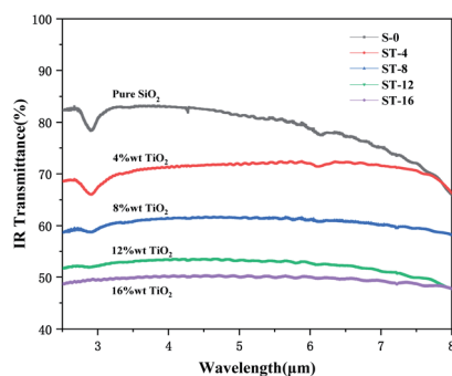
Fig. 6 Infrared transmittance curves of samples with different \text{TiO}_2 content.
