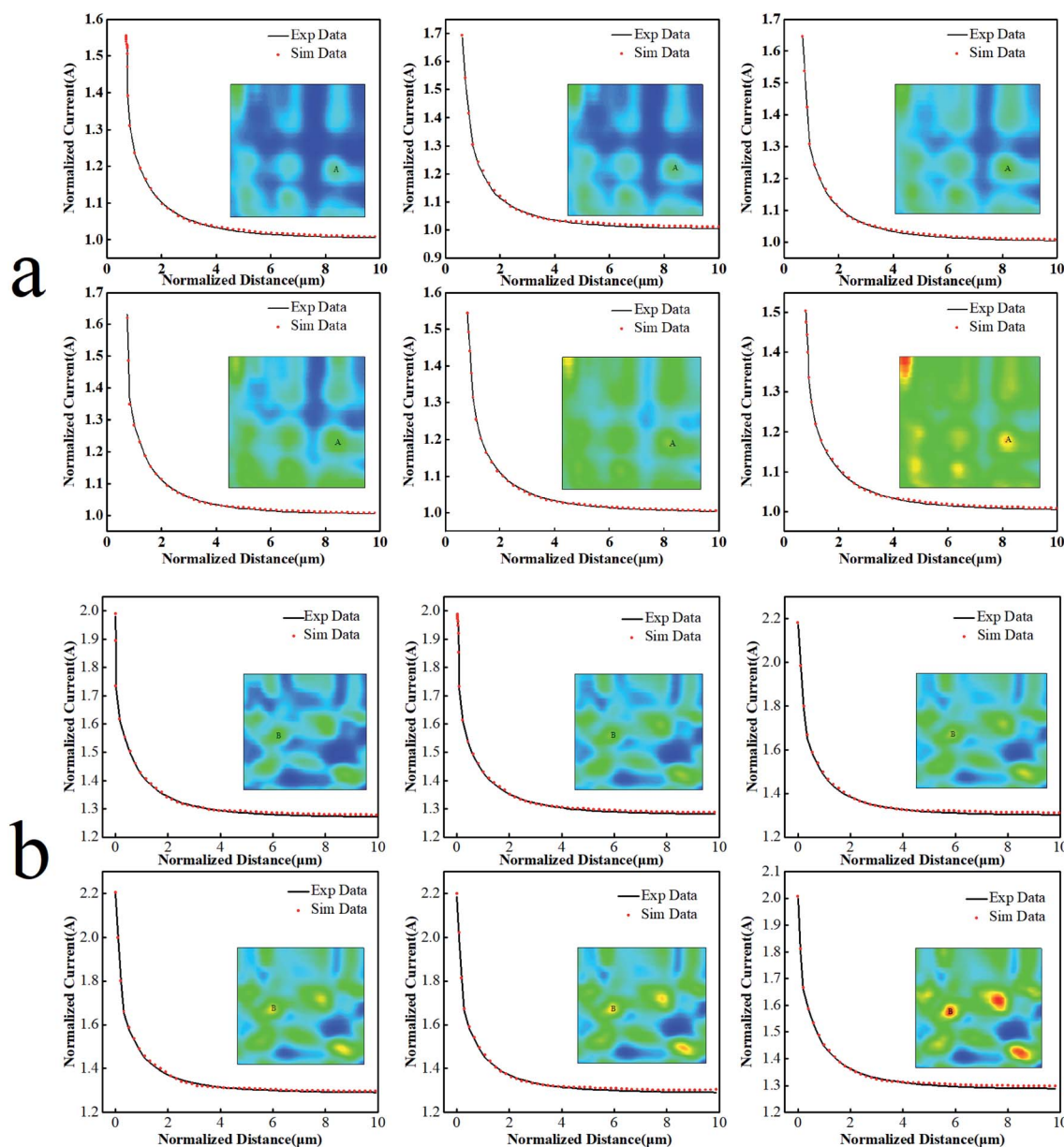
Fig. 6 The UME probe approach curve with (a) the PbO 2 -Co 3 O 4 -MnO 2 electrode and (b) the traditional PbO 2 electrode, E_t = 0.05 V, E_s = 0.1 – 1.0 V, increment distance = 1 μm, quiet time = 60 s.
