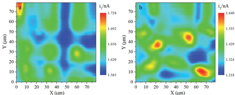
Fig. 3 SECM map of the 80 \mu\text{m} \times 80 \mu\text{m} constant-height surface at the open circuit potential of (a) the \text{PbO}_2\text{-Co}_3\text{O}_4\text{-MnO}_2 electrode and (b) the traditional \text{PbO}_2 electrode, d = 3 \mu\text{m} .
