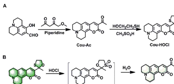
Scheme 1 (A) Synthesis of Cou–HOCl. (B) Reaction of Cou–HOCl with HOCl.
