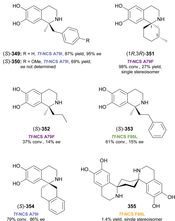
Fig. 5 Examples of 1,1-disubstituted and spirocyclic tetrahydroindoles obtained by NCS reactions of open-chain or cyclic ketones.
