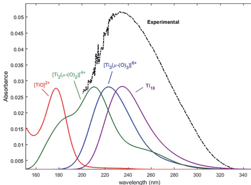
Fig. 8 Comparison of the normalized convolution of the excitation energies calculated by TD-DFT for \text{TiO}_2^+ , [\text{Ti}_2(\mu\text{-(O)}_2)]^{4+} , [\text{Ti}_3(\mu\text{-(O)}_3)]^{6+} and \text{Ti}_{18} with the experimental UV-vis spectrum of titanium(IV) in nitric acid from Fig. 1b.
