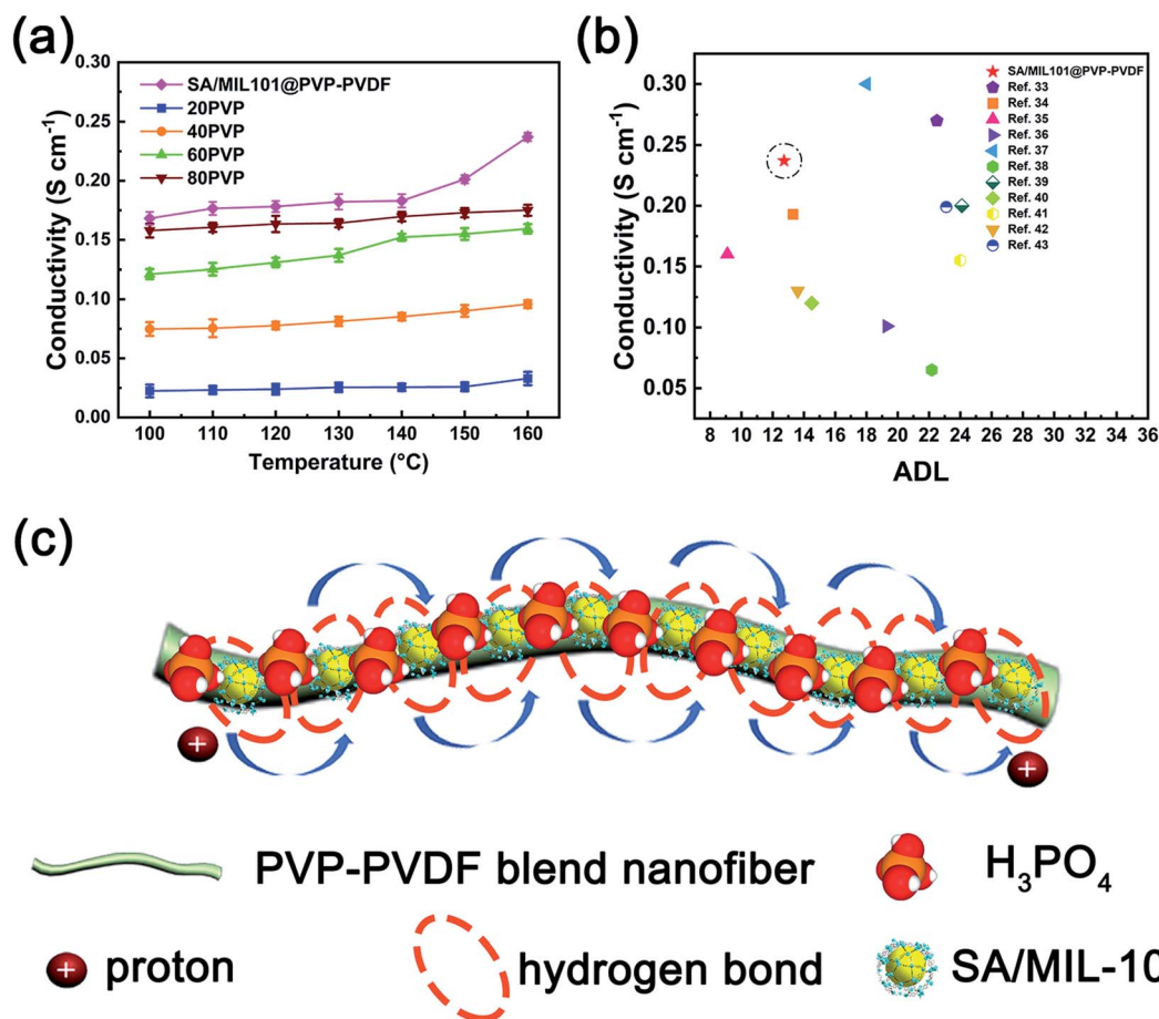
Fig. 7 (a) Proton conductivities of membranes after PA doping. (b) Comparative analysis of conductivity ( 160^{\circ}\text{C} ) vs. ADL of SA/MIL101@PVP-PVDF and some reported PA-doped membranes. (c) Schematic illustration of the possible proton conducting mechanism of PA-doped SA/MIL101@PVP-PVDF.
