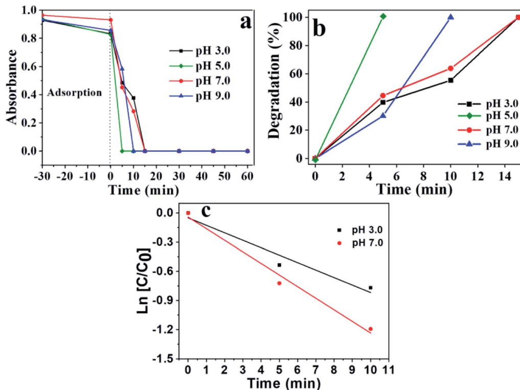
Fig. 2 (a) Influence of pH on ibuprofen photodegradation; (b) ibuprofen (10 -4 M) degradation rate versus irradiation time for the different pHs; (c) pseudo-first order reaction for ibuprofen degradation.
