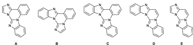
Scheme 1 Trinuclear N-fused hybrid scaffolds.
