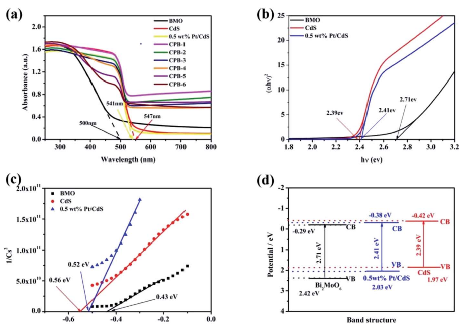
Fig. 5 (a) UV-Vis diffuse reflectance spectra of CdS, Bi 2 MoO 6 , Pt/CdS, and CPB composites with different compositions. (b) Plots of (\alpha h\nu)^2 versus h\nu used to estimate the optical band gaps of CdS, Pt/CdS, and Bi 2 MoO 6 . (c) Mott-Schottky plots of CdS, Pt/CdS, and Bi 2 MoO 6 . (d) Band structures of CdS, Pt/CdS, and Bi 2 MoO 6 .
