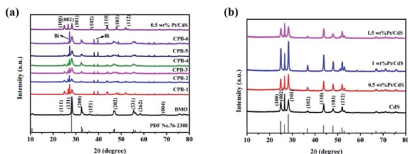
Fig. 1 XRD patterns of (a) CdS NRs, Bi 2 MoO 6 NSs, 0.5 wt% Pt/CdS, and a series of ternary CPB composites (b) a series of Pt/CdS composites.
