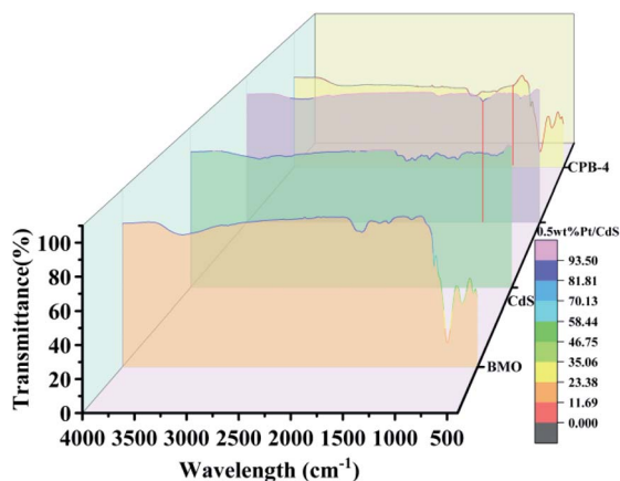
Fig. 6 FT-IR spectra of Bi 2 MoO 6 , CdS, Pt/CdS, and CPB-4 composite.
