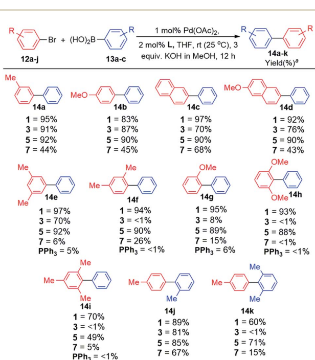
Scheme 2 Substrate scope evaluation. Reaction conditions: ArBr (1 equiv.), ArB(OH) 2 (1.5 equiv.), 2 M KOH in MeOH (3 equiv.), Pd(OAc) 2 (1 mol%), L (2 mol%), THF, Ar, 12 h, rt. a Isolated yields from an average of two runs with <5% deviation. GC results included in Tables S5 and S6 (ESI†).
