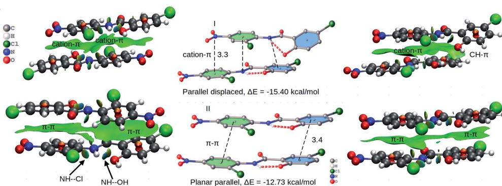
Fig. 4 (a) The formation of a stable aggregated system of niclosamide with 14 monomers. The aggregation is a multi-step process whereby individual monomers bind to form small aggregates dominated by the formation of parallel and T-shape conformations. With time, the small aggregates join to form a large cluster and re-orient to build a stable planar anti-parallel displaced conformation. (b) MEP surface of niclosamide, the energies shown at different points are in kcal mol -1 . (c and d) Interactions and arrangements of niclosamide dimers, the distance shown is in Å. To the right side of each figure is the NCI plot showing the interactions.
