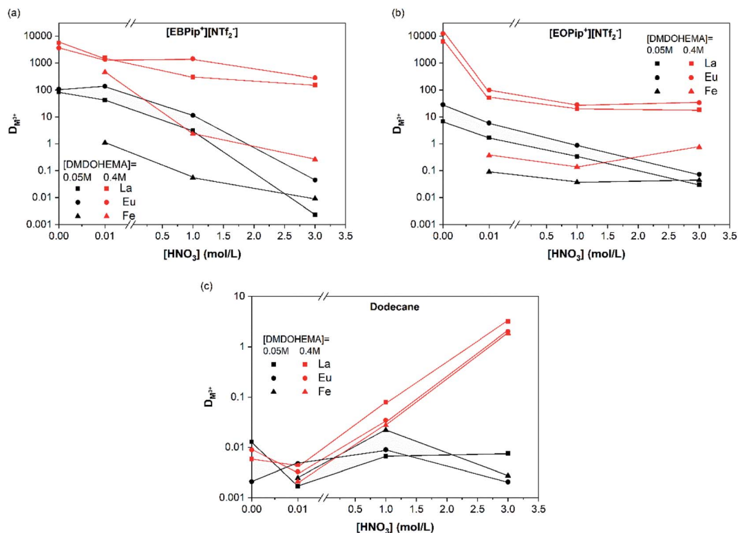
Fig. 3 Distribution coefficients as a function of the nitric acid concentration for [DMDOHEMA] = 0.05 M (black symbols) and 0.4 M (red symbols), in: (a) [EBPip + ] [NTf 2 - ], (b) [EOPip + ] [NTf 2 - ] and (c) dodecane.
