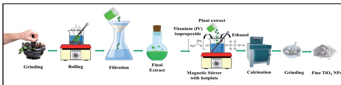
Fig. 1 The schematic diagram of the complete process involving 'green-synthesis' of TiO 2 NPs.
