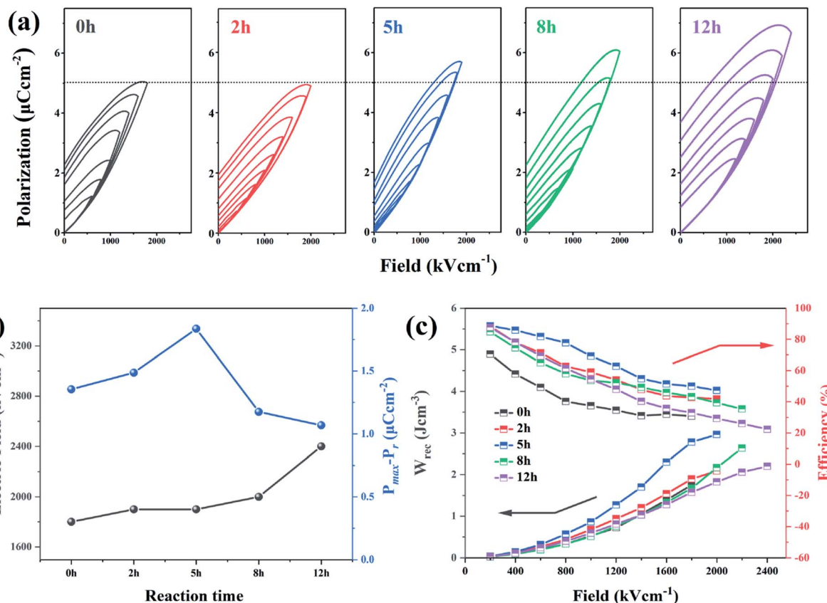
Fig. 7 (a) Hysteresis loops, (b) breakdown strength and P_{\text{max}} - P_r values (c) discharged energy density ( W_{\text{rec}} ) and efficiency ( \eta ) of dehydrofluorinated PVDF fiber membranes with varying reaction times.
