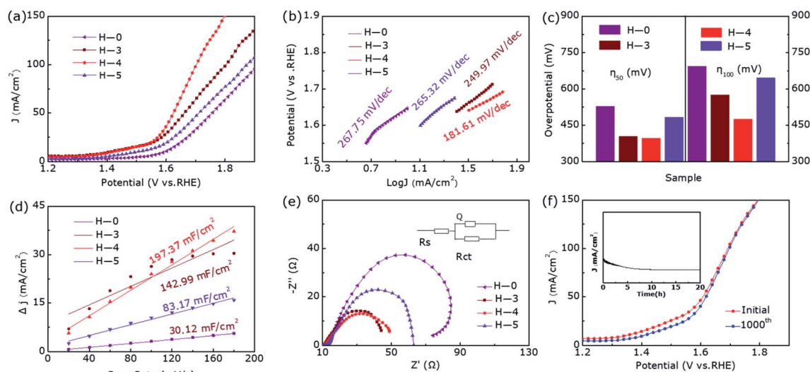
Fig. 3 (a) The LSV curves, (b) Tafel plots and (c) \eta_{50} and \eta_{100} of H-0, H-3, H-4 and H-5 for the OER. (d) The C_{dl} and (e) EIS Nyquist plots of all samples. (f) LSV curves of H-4 catalyst before and after 1000 cycles; the inset shows the chronoamperometry test of sample H-4.
