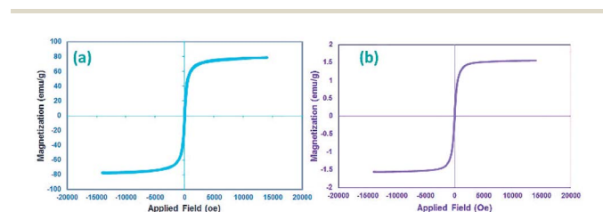
Fig. 2 VSM curves of the (a) CoFe 2 O 4 and (b) N-GQDs/CoFe 2 O 4 magnetic nanocomposite.
