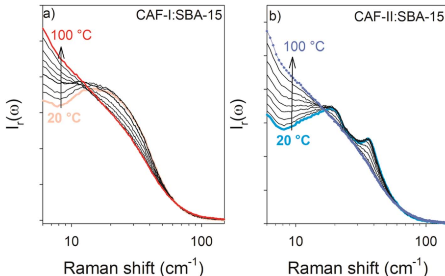
Fig. 4 I_r(\omega) -spectra collected during a first heating ramp at 1\text{ }^\circ\text{C min}^{-1} of freshly prepared composites plotted by step of 10\text{ }^\circ\text{C} in the 20\text{--}100\text{ }^\circ\text{C} range corresponding to the first exothermic transformation; spectra of (a) CAF-I:SBA-15 (b) CAF-II:SBA-15. The arrows show the increase of the quasielastic intensity highlighting the disordering nature of the exothermic transformation. A logarithm \omega -scale was used for a clear representation of spectral changes at very low-frequencies.
