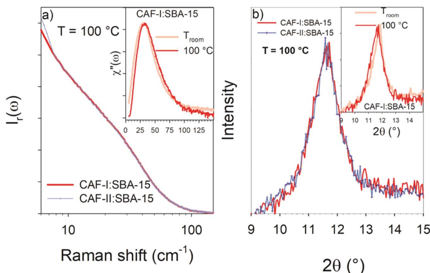
Fig. 5 Analysis of the physical state of the two composites at 100\text{ }^\circ\text{C} , from (a) LFRS plotted in reduced intensity ( I_r(\omega) -spectra) using a logarithm \omega -scale for a better analysis of the low-frequency range; Raman susceptibilities collected in the CAF-I:SBA-15 composite are plotted in the inset on either side of the exothermic transition at room temperature and 100\text{ }^\circ\text{C} (b) PXRD plotted in the 9\text{--}15\text{ }2\theta -region corresponding to the broadened 110 Bragg peak of CAF-I; data collected in the CAF-I:SBA-15 composite are plotted in the inset on either side of the exothermic transition at room temperature and 100\text{ }^\circ\text{C} .
