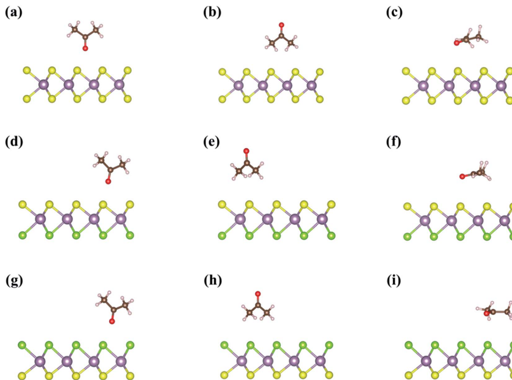
Fig. 2 Optimized adsorption structures of acetone on the TMDs monolayers without the external electric fields: (a) \text{Ace}_{\text{v1}} , (b) \text{Ace}_{\text{v2}} , and (c) \text{Ace}_{\text{h}} on \text{MoS}_2 ; (d) \text{Ace}_{\text{v1}} , (e) \text{Ace}_{\text{v2}} , and (f) \text{Ace}_{\text{h}} on S-layer of the Janus \text{MoSSe} ; (g) \text{Ace}_{\text{v1}} , (h) \text{Ace}_{\text{v2}} and (i) \text{Ace}_{\text{h}} on Se-layer of the Janus \text{MoSSe} . Purple, yellow, and green spheres represent Mo, S, and Se atoms, respectively, while brown, red, and light pink balls are C, O, and H atoms, respectively.
