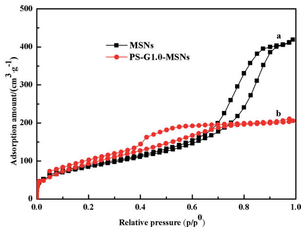
Fig. 2 \text{N}_2 adsorption-desorption isotherms of the synthesized MSNs (a) and PS-G1.0-MSNs (b) sorbents.
