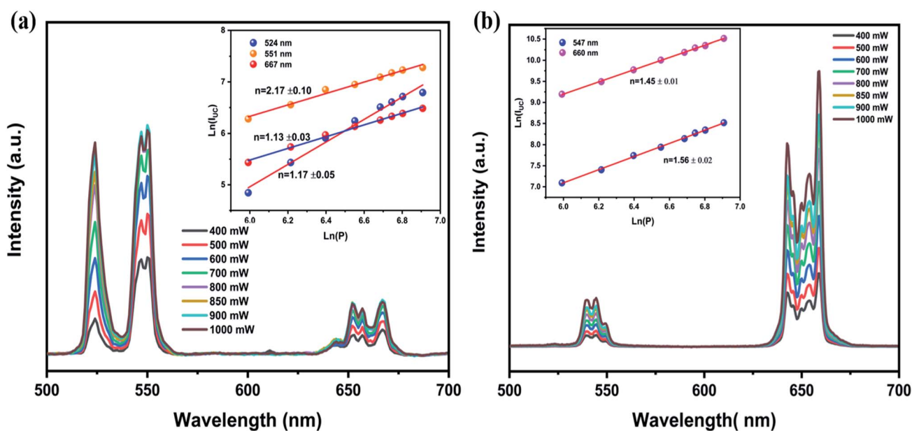
Fig. 7 Represents the variation UC emission at different pump powers, inset shows the dependences of \ln(I_{\text{UC}}) on \ln(P) : (a) for \text{LiZnPO}_4:\text{Er}^{3+}/\text{Yb}^{3+} . (b) For \text{LiZnPO}_4:\text{Ho}^{3+}/\text{Yb}^{3+} .
