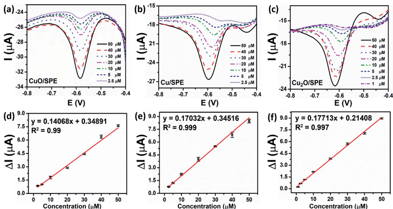
Fig. 6 DPV curves of CuO-NPs/SPE (a), Cu-NPs/SPE (b), and Cu 2 O-NPs/SPE (c) in 0.1 M PBS (pH 5) containing CAP (1–50 \mu\text{M} ) at a scan rate of 6 \text{ mV s}^{-1} , corresponding to the calibration plots between peak current vs. various concentrations of CAP (d–f), along with error bars.
