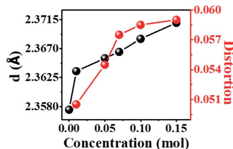
Fig. 10 MYAS:x \text{Dy}^{3+} : changes in bond length and twist of Y/Mg(1) \text{O}_6 .
