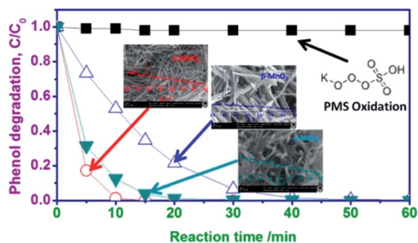
Fig. 16 Phenol degradation of MnO 2 -based nanomaterials with different phase structures. Reproduced by Saputra et al. 29 with permission from ACS.
