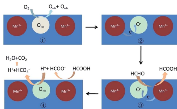
Fig. 17 The possible mechanism of catalytic oxidation of HCHO to CO 2 on partially crystallized mesoporous MnO x under dry condition. Reproduced by Guan et al. 173 with permission from Elsevier.
