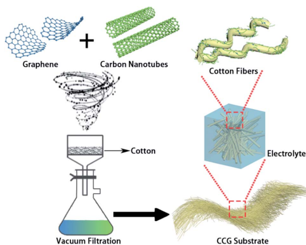
Fig. 1 Schematic of the CCG substrate preparation and its corresponding configurations.
