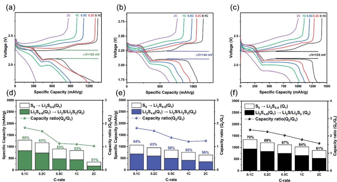
Fig. 5 Charge and discharge specific capacity versus voltage profiles of the (a) CC, (b) CG, (c) CCG substrate batteries from 0.1C to 2C. Capacity contribution of lower potential ( \text{Q}_1 ) and higher potential ( \text{Q}_2 ) and the \text{Q}_2/\text{Q}_1 ratio at various C rates for the (d) CC, (e) CG, (f) CCG substrate batteries.
