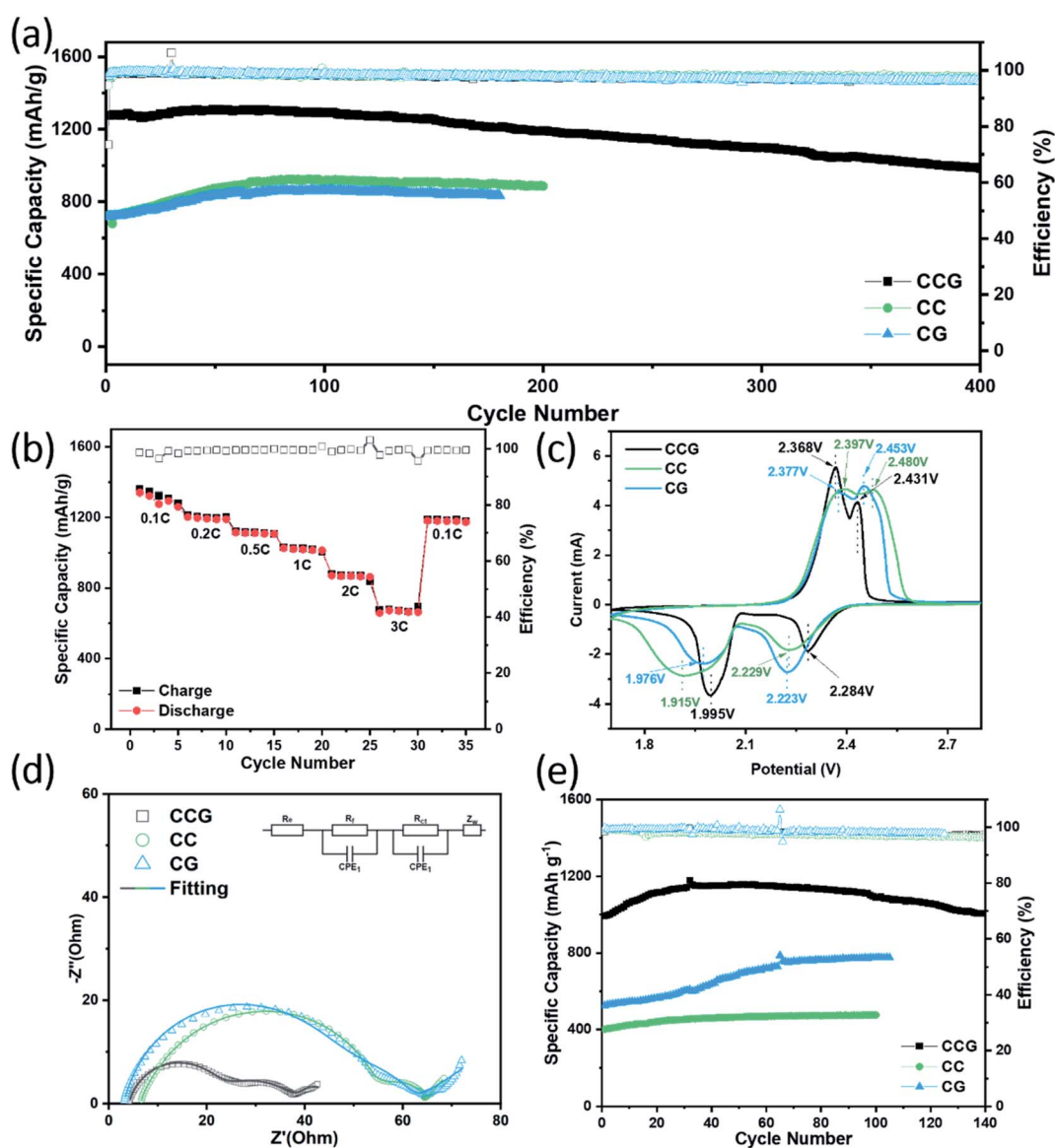
Fig. 4 (a) Cycling performances of the batteries with different substrates with a low sulfur loading at a current density of 1 \text{ C} , (b) rate performances of the battery with CCG substrate, (c) CV of CC, CG, CCG substrates batteries at a scan rate of 0.1 \text{ mV s}^{-1} , respectively, (d) EIS profiles of Li-S batteries using CC, CG and CCG substrates, (e) cycling performances of the batteries with different substrates with a high sulfur loading at a current density of 0.5 \text{ C} .
