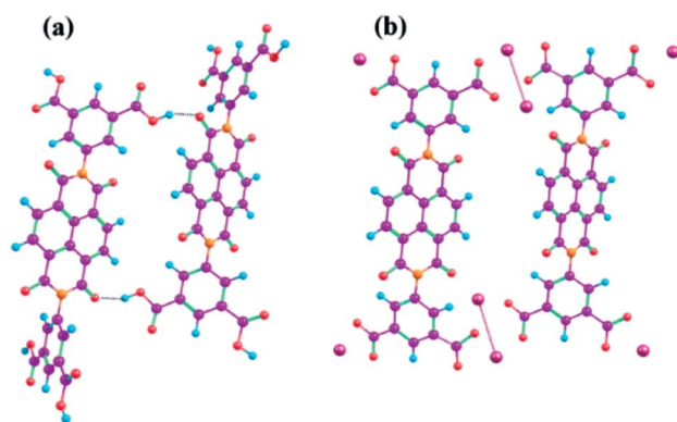
Fig. 2 Optimized geometry of N1 and N2 dimer model (a) showing H-bonding, and (b) absence of H-bonding, respectively, generated in ChemCraft software.
