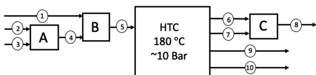
Fig. 10 Block Flow Diagram of Chirside's theoretical HTC plant for food and sewage waste; (1) the food waste (FW); (2) the wet faecal sludge (FS); (3) the sewage water (SW) used to transport the faecal sludge (100% water); (A) where streams 2 and 3 are mixed during transport to the plant, resulting in; (4) Primary Sewage Sludge (PSS), which is wet faecal sludge and sewage water (FS + SW); (B) where streams 1 and 4 mix before entering the HTC plant, resulting in; (5) primary sewage sludge and food waste (dry biomass/water ratio= 0.145); (6) the hydrochar produced by HTC of the faecal sludge (HC FS ); (7) the hydrochar produced by the HTC of the food waste (HC FW ); (C) where the properties of streams 6 and 7 are “mixed” to result in an average hydrochar of the two streams, resulting in; (8) mixed hydrochar (HC mix ); (9) process water (PW eff ) after separation of the solid hydrochar, and; (10) the organic fraction (ORG) which remains in either the process water as aqueous chemicals or is produced as effluent gas such as CO 2 , CO, CH 4 .
