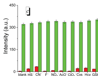
Fig. 5 UV-vis absorption (a) and fluorescence spectra (b) of PI-CN (15 \mu\text{M} ) in the presence of 1.0 equiv. of various species ( \text{HS}^- , \text{CN}^- , \text{F}^- , \text{NO}_2^- , \text{AcO}^- , \text{ClO}_4^- ) and 50 equiv. of common sulphur compounds (Cys, Hcy, and GSH) in EtOH/PBS (v/v 1 : 3, pH 7.4) recorded after 12 min. Inset: fluorescence enhancement of PI-CN (15 \mu\text{M} ) with or without various species (1.0 equiv.) at 499 nm. (c) Competing response of probe PI-CN (15 \mu\text{M} ) towards various species (1 equiv.) in EtOH/PBS (v/v 1 : 3, pH 7.4). The red bars represent the addition of one of the various species to the solution of the probe; the green bars represent the fluorescence intensity of the probe in the presence of various species, then added \text{HSO}_3^- after 12 min.
