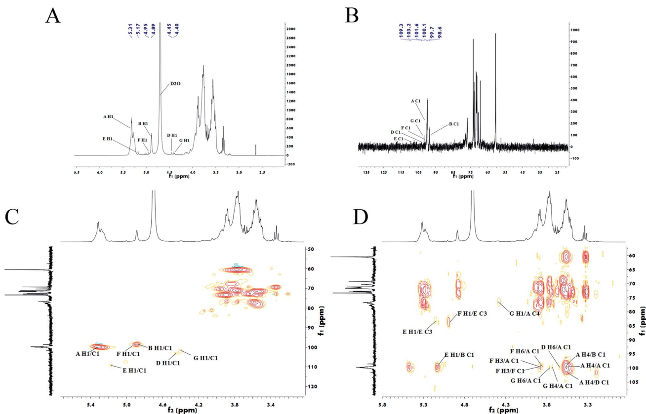
Fig. 4 Nuclear magnetic resonance analysis of PLB-1-1. 1 H (A), 13 C (B), HSQC (C) and HMBC (D) spectra of PLB-1-1.
