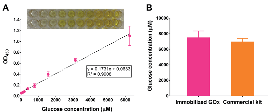
Fig. 8 (A) Glucose assay conducted in GOx-immobilized 96-well plates. A calibration curve was obtained by plotting the absorbance of the yellow TMB product at 450 nm versus glucose concentration. Each concentration was assayed in duplicate. Linear regression analysis was performed using GraphPad Prism 7. Top: representative image of a GOx-immobilized 96-well plate after conducting the glucose assay; (B) Average plasma glucose concentrations from three different healthy rats assayed using the developed glucose assay platform and compared to a commercial glucose assay kit.
