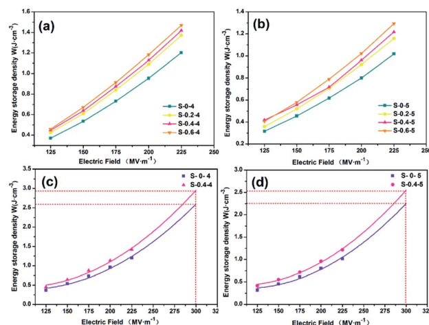
Fig. 11 The actual values of the energy storage density of the materials which were calculated based on the integration of the D - E loops measured by the experimental apparatus: (a) and (b) energy storage density; (c) and (d) curve fitting of energy storage density.
