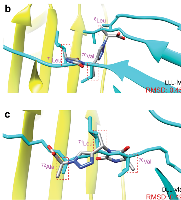
Fig. 1 (a) NEDD8 is clenched at its C-terminus by a fist formed from NAE, which consists of UBA3 (yellow) and APPBP1 (red). (b and c) Overlay of the featured chemotypes on 8 Leu, 70 Val, 71 Leu, 72 Ala of NEDD8 (see Fig. S1† for all overlays).
