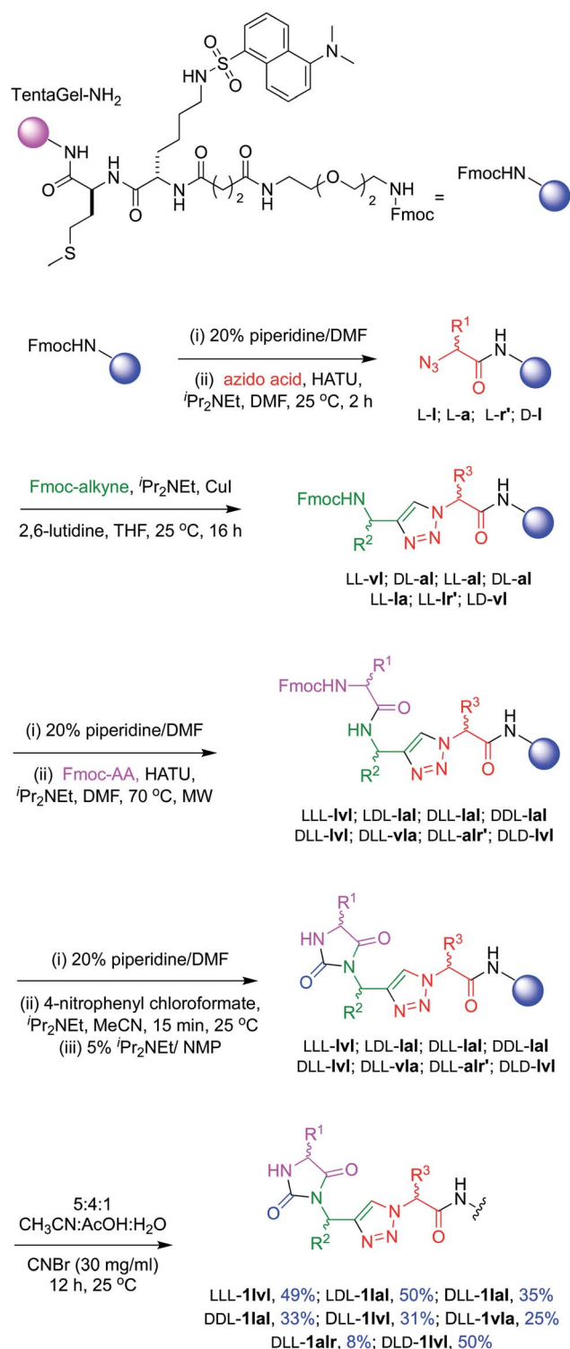
Scheme 1 Solid phase syntheses of chemotypes 1. In this route, LLD-1r'Ia was made slightly differently insofar as the final supported material was treated with 95 : 2.5 : 2.5 TFA : H 2 O : HSiEt 3 for 2 h to remove the Mtr protecting group before CNBr cleavage.
