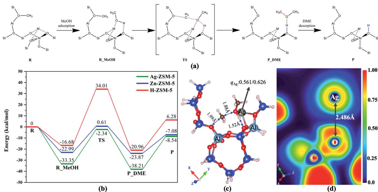
Fig. 6 (a) Reaction scheme and (b) potential energy surface of M-ZSM-5–MeOH + MeOH ( -\text{OMe}^+ via a rapid dehydration of \text{MeOH}_2^+ over BAS) \rightarrow M-ZSM-5 + DME ( M = \text{Ag}, \text{Zn} and \text{H} ), (c) transition state (TS) structure and charge value of Ag ( q_{\text{M}} ) for R_MeOH and for TS, (d) electron localization function (ELF) contour of (c).
