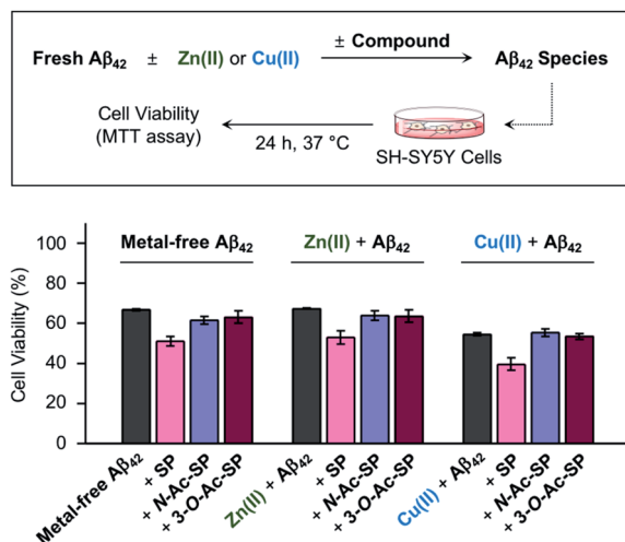
Fig. 8 Effect of SP, N-Ac-SP , and 3-O-Ac-SP on the toxicity induced by metal-free A\beta_{42} or metal- A\beta_{42} in living cells. Cell viability, determined by the MTT assay, was calculated in comparison to that of the cells treated with an equivalent amount of the buffered solution with 0.2% v/v DMSO (20 mM HEPES, pH 7.4 or pH 6.8, 150 mM NaCl). Error bars indicate the standard error from three independent experiments. Conditions: [A\beta_{42}] = 10 \mu\text{M} ; [Zn(II) or Cu(II)] = 10 \mu\text{M} ; [compound] = 10 \mu\text{M} (0.2% v/v DMSO); 20 mM HEPES, pH 7.4 [for metal-free and Zn(II)-containing samples] or pH 6.8 [for Cu(II)-containing samples], 150 mM NaCl.
