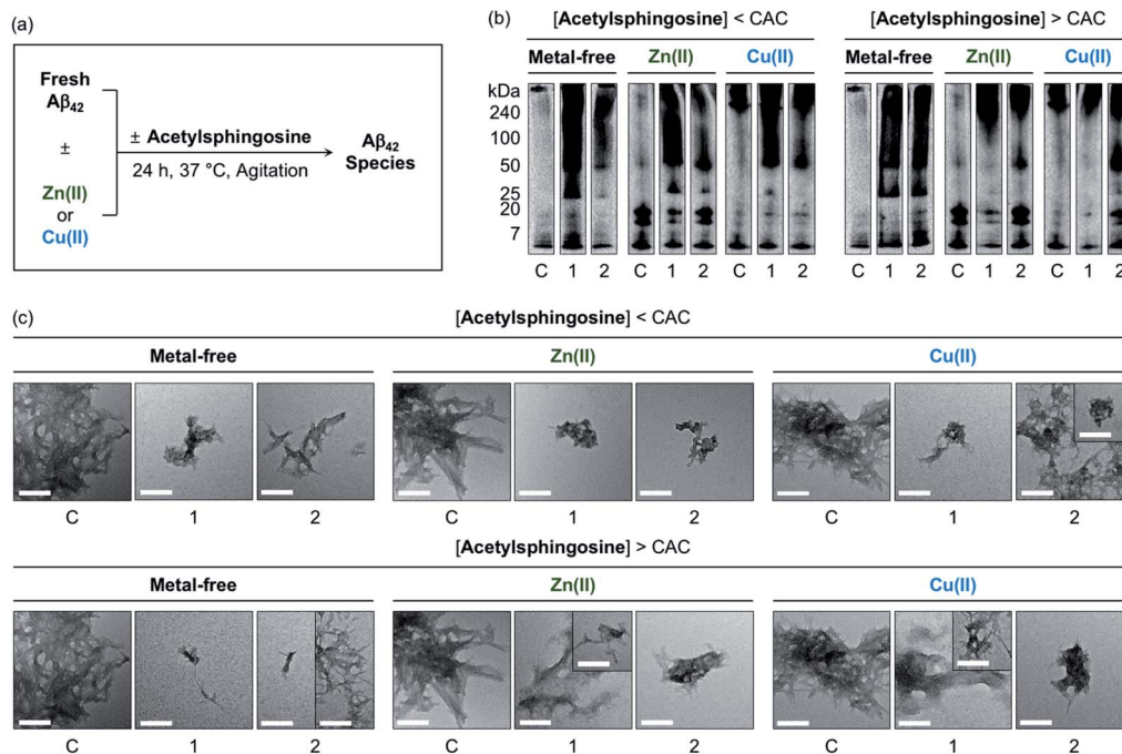
Fig. 7 Influence of N-Ac-SP and 3-O-Ac-SP on the aggregation of metal-free A\beta_{42} and metal- A\beta_{42} . (a) Scheme of A\beta_{42} aggregation experiments. (b) Analysis of the size distribution of the resultant A\beta_{42} species by gel/Western blot using an anti- A\beta antibody (6E10). Lanes: (C) A\beta_{42} \pm Zn(II) or Cu(II); (1) C + N-Ac-SP ; (2) C + 3-O-Ac-SP . The original gel images are shown in Fig. S13† (c) Morphologies of the resultant A\beta_{42} aggregates from (b) detected by TEM. Conditions: [A\beta_{42}] = 25 \mu\text{M} ; [Zn(II) or Cu(II)] = 25 \mu\text{M} ; [acetylsphingosine] = 10 \mu\text{M} (below the CAC) or 100 \mu\text{M} (above the CAC) (1% v/v DMSO); 20 mM HEPES, pH 7.4 [for metal-free and Zn(II)-containing samples] or pH 6.8 [for Cu(II)-containing samples], 150 mM NaCl; 37 °C; 24 h; constant agitation. Scale bars = 200 nm.
