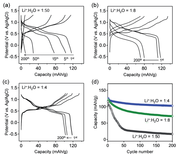
Fig. 3 Charge/discharge curves of \text{VOPO}_4 \cdot n\text{H}_2\text{O} electrodes with aqueous \text{Li}^+ electrolytes. The \text{Li}^+ : \text{H}_2\text{O} ratios are (a) 1 : 50 (LiTFSI/50 \text{H}_2\text{O} ), (b) 1 : 8 (LiTFSI/8 \text{H}_2\text{O} ), and (c) 1 : 4 (LiTFSI/4 \text{H}_2\text{O} ), respectively. The specific current is 1 \text{ A g}^{-1} . (d) Capacity retention during 200 charge/discharge cycles.
