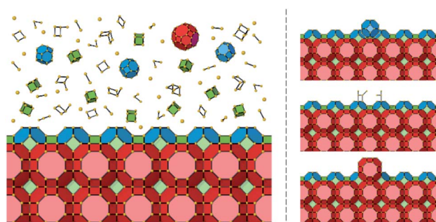
Fig. 6 Left: The (100) face of a zeolite A crystal shown as natural tiles surrounded by closed cages (bottom) immersed in a mother solution (top). The species formed in solution/gel is a mixture of monomers, dimers, n-mers, rings and cages/tiles. Right: Three potential growth options for a surface. An incorrect cage or structure could grow through several growth or dissolution steps (top), this cage will not match the underlying crystal structure at the surface and would preferentially dissolve. Another cage could partially grow through several steps (centre) but would also prefer to dissolve until forming a complete cage/tile. Finally, the correct tile could grow through several steps (bottom). Once this tile is fully formed it would persist due to its metastability and its formation would be a rate-determining step in crystal growth.
