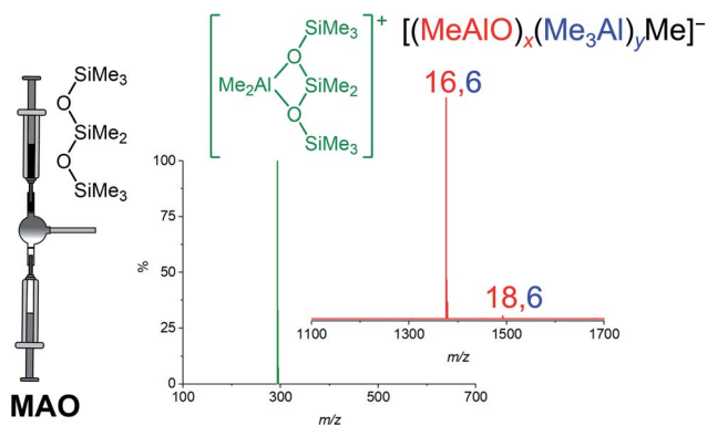
Fig. 1 Ionization of MAO to generate [\text{Me}_2\text{Al}(\text{OMTS})]^+ (green) and predominantly [\mathbf{16},\mathbf{6}]^- with small amount of [\mathbf{18},\mathbf{6}]^- .
