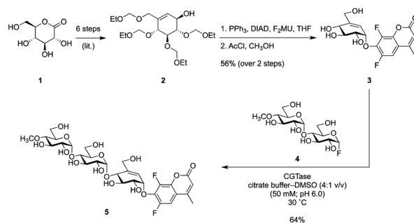
Scheme 1 Synthesis of titration reagent 5 .
