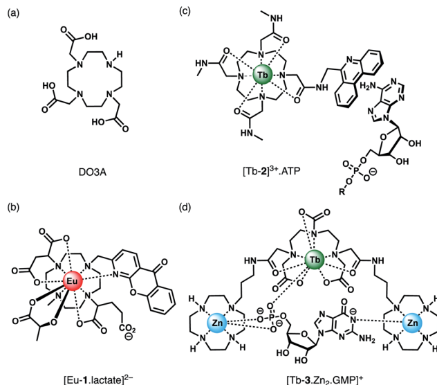
Fig. 4 (a) Common macrocyclic ligand DO3A; (b)–(d) examples of Ln(III) receptors that utilise different mechanisms of anion binding.
