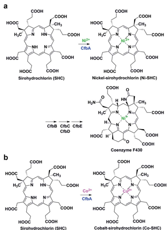
Fig. 1 CfbA-catalyzed chelate reactions with substrate SHC. (a) Insertion of \text{Ni}^{2+} into SHC in the coenzyme F430 biosynthetic pathway. (b) Insertion of \text{Co}^{2+} into SHC, which has been characterized using Methanosarcina barkeri CfbA. 3,18
