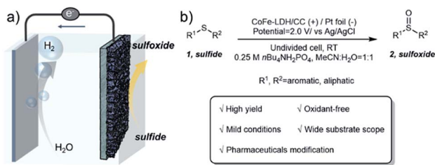
Fig. 1 (a) Electrocatalytic oxidation of sulfides 1 coupled with the HER. (b) Oxidation of sulfides 1 to form sulfoxides 2.
