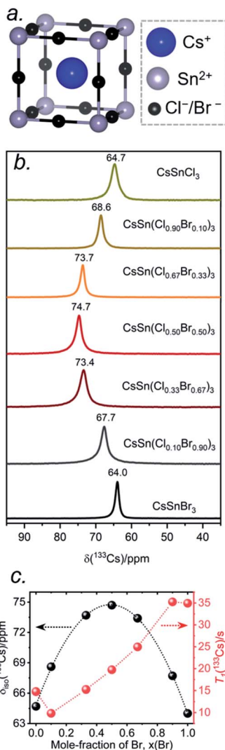
Fig. 5 (a) Local cuboctahedral environment of 12 halogen atoms around the Cs atom. (b) Room temperature ^{133}\text{Cs} NMR spectra for \text{CsSn}(\text{Cl}_{1-x}\text{Br}_x)_3 , acquired at 11.75 T with a magic-angle spinning frequency of 13 kHz. (c) Plots of \delta_{\text{iso}}(^{133}\text{Cs}) and ^{133}\text{Cs} T_1 values as a function of Br content. The \delta_{\text{iso}} plot was fit to the equation \delta_{\text{iso}}(^{133}\text{Cs})/\text{ppm} = 64.8 + 40.6x - 41.5x^2 ( R^2 = 0.999 ).
