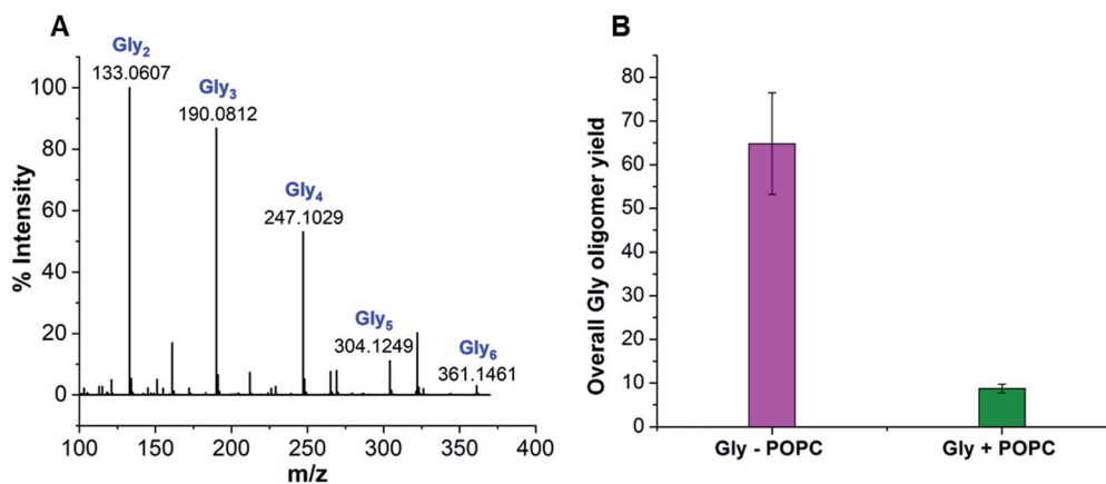
Fig. 1 Formation of Glycine oligomers under wet–dry cycles and the effect of POPC on their overall yield as analysed by LC-MS. (A) Upon five wet–dry cycles at 90 °C, 80 mM Gly solution shows the formation of Glycine oligomers of up to 6-mers. (B) Relative abundances of individual oligomers are summed up to give the overall oligomer yield, which was found to be lower in the presence of POPC (Gly + POPC) than that of the Gly control (Gly – POPC) reaction. All glycine peptides were detected and quantified using LC-MS (see Methods for more details). The error bars represent standard deviation ( N = 4 ).
