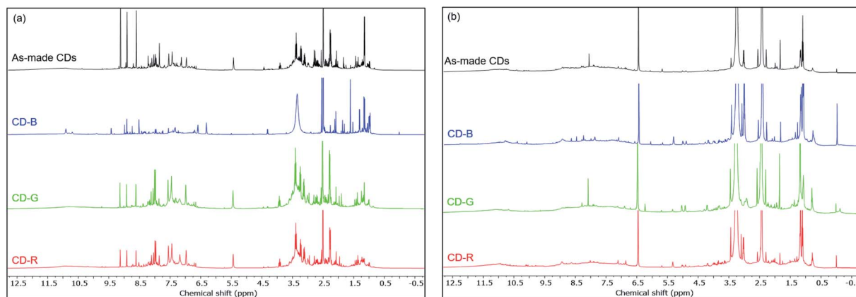
Fig. 4 1 H NMR spectra of as made CDs, CD-B, CD-G, and CD-R in DMSO-d 6 before dialysis (a) and after dialysis (b).
