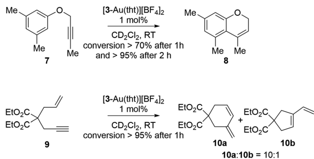
Scheme 5 Intramolecular hydroarylation and enyne cyclization reactions catalyzed by [3-Au(tht)][BF 4 ] 2 .
