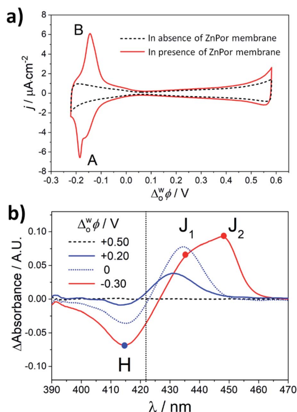
Fig. 2 (a) Cyclic voltammetry (CV) in the absence and presence of the ZnPor membrane in the configuration presented schematically in Fig. 1a. The scan rate was 25 mV s^{-1} . The 4-electrode electrochemical cell setup used for these measurements is presented in Fig. S1.† (b) Differential TIR-UV/vis absorbance spectra of the ZnPor membrane at different \Delta\phi^w . The spectrum of the membrane at +0.50 V was taken as a blank.
