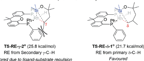
Scheme 6 Hartwig's intramolecular dehydrogenative silylation via 7-membered rhodacycles.
