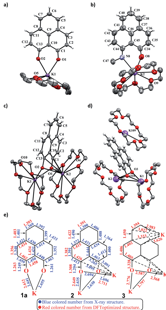
Fig. 1 (a) X-ray crystallographic structure of 1a(CE). Ellipsoids are shown at 50% probability, selected bond lengths ( \text{\AA} ) and bond angles [deg]: K1–O1 2.6414, K1–O2 2.6551, O1–C1 1.2613, O2–C13 1.2490, O1–K1–O2 63.2271; (b) X-ray crystallographic structure of 1b(CE). Ellipsoids are shown at 50% probability, selected bond lengths ( \text{\AA} ) and bond angles [deg]: K2–O8 2.5976, K2–N8 2.8418, O8–C34 1.2550, N8–C44 1.2939, O8–K2–N8 60.9823, K2–O8–C34 147.4870, K2–N8–C44 139.1102; (c) X-ray crystallographic structure of 2. Ellipsoids are shown at 50% probability, selected bond lengths ( \text{\AA} ) and bond angles [deg]: K1–O1 2.6289, K1–O2 2.6350, O1–C1 1.2943, O2–C13 1.2955, K1–O1–K2 95.9253, K1–O2–K2 95.8503; (d) DFT optimized structure of 3. A few selected bond lengths ( \text{\AA} ) and bond angles [deg]: K1–K2 4.0573, K1–O3–K2 97.7281; (e) bond distance analysis of 1a(CE), 2 and 3 by X-ray structure and DFT study.
