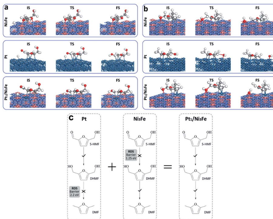
Fig. 5 The tandem mechanism of Pt and the Ni 3 Fe interface. Optimized structures of reaction intermediates for the first hydrogenation step (a) and the dehydroxylation of MFA (b) over Pt, Ni 3 Fe and the Pt 1 /Ni 3 Fe surface. (c) Tandem mechanism on Pt/Ni 3 Fe, combining the catalytic performance of both Pt and Ni 3 Fe catalysts. The light blue, orange, blue, grey, red and white spheres represent Ni, Fe, Pt, C, O and H atoms, respectively.
